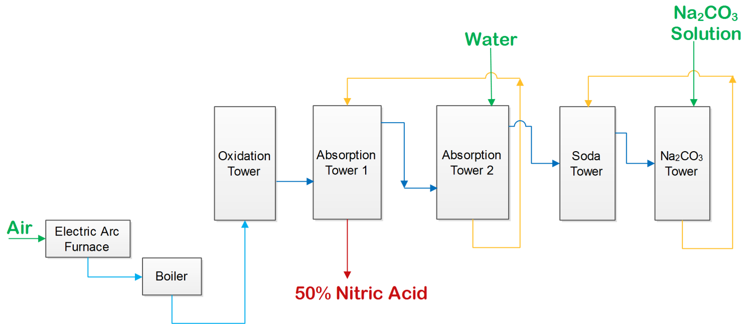
Figure: Manufacturing of Nitric Acid by Arc Process
